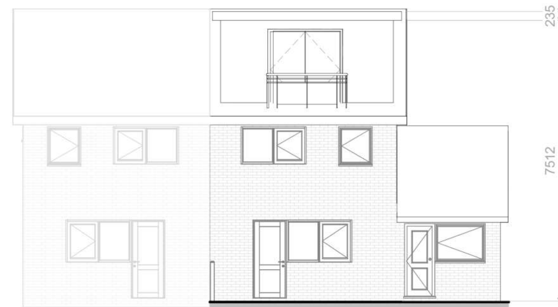
Proposed Elevation-Rear
