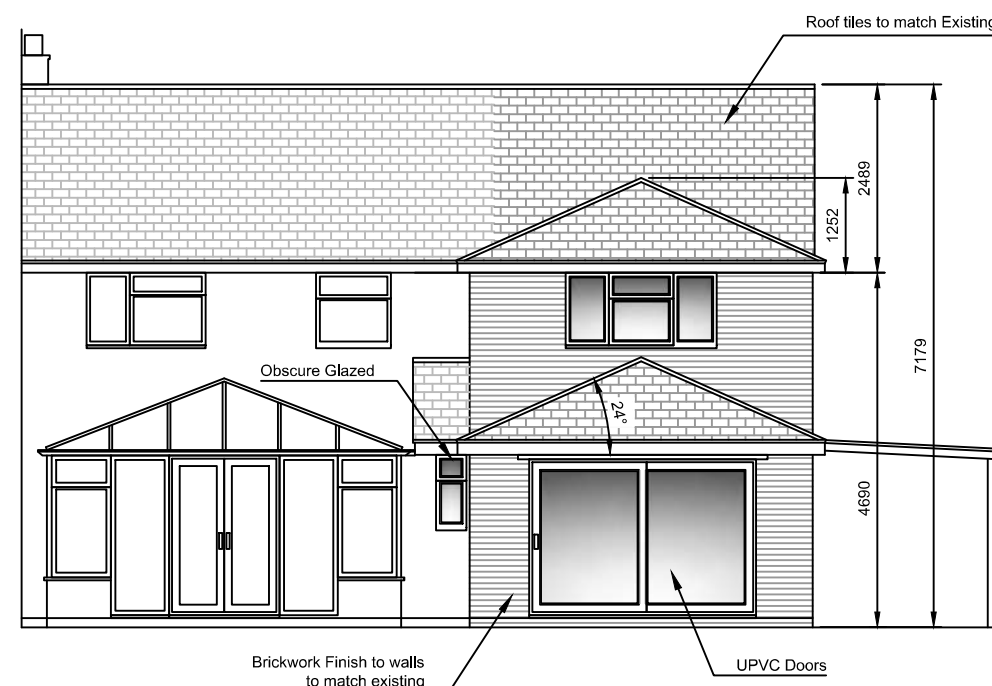
Rear Elevation
