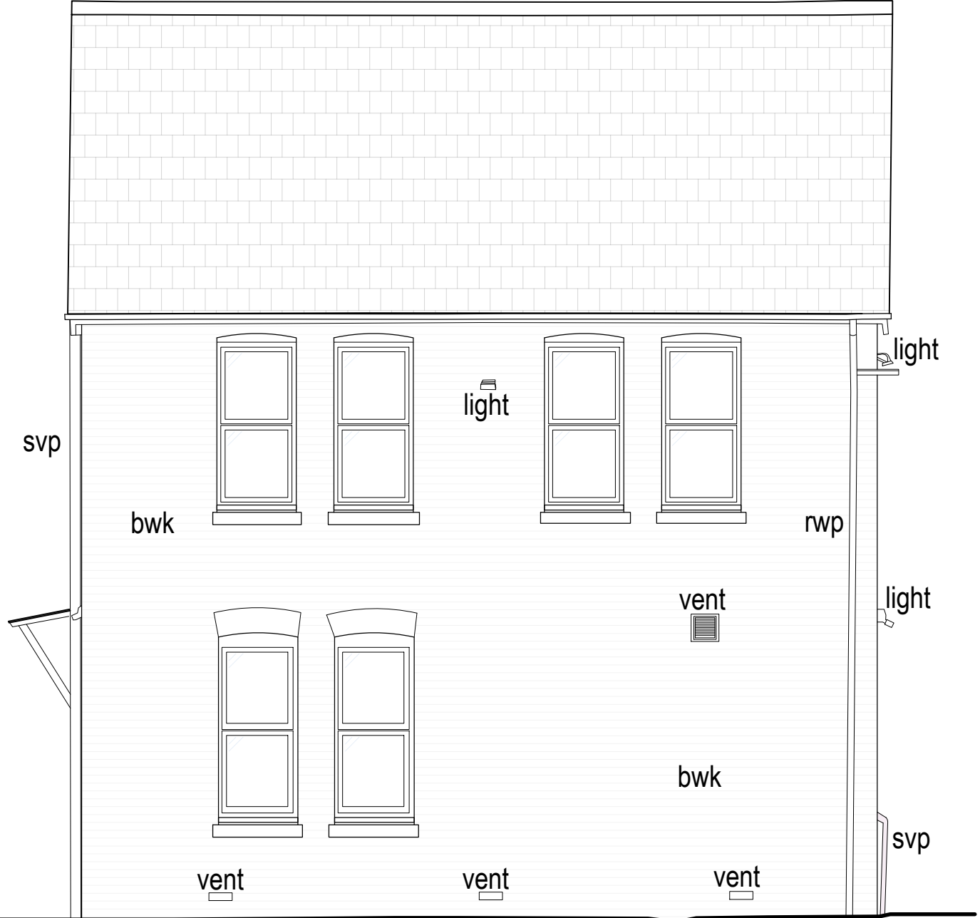
East Elevation
