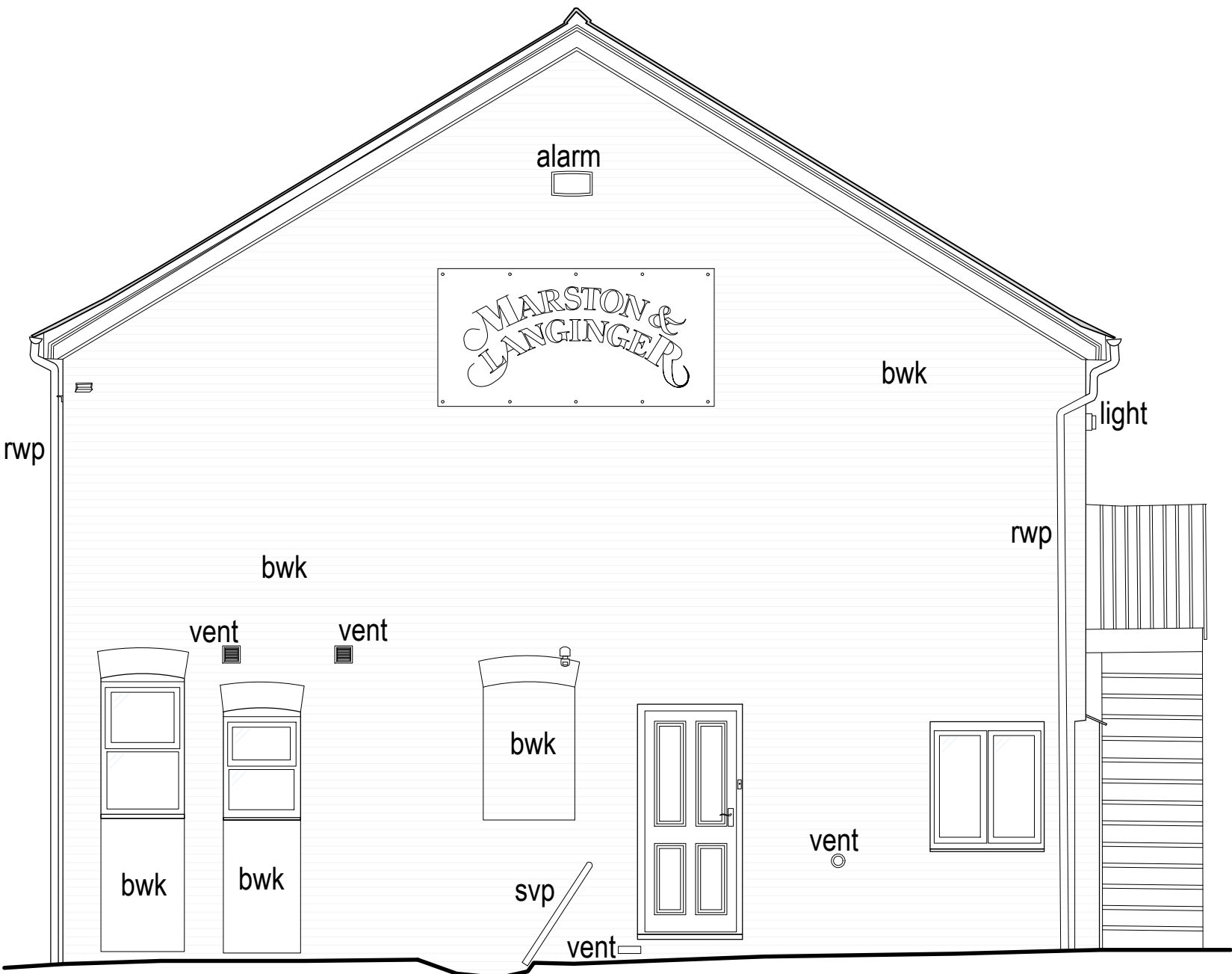
North Elevation
