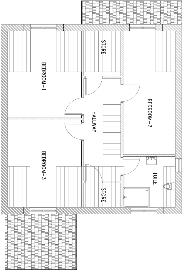
2 EXISTING FIRST FLOOR SCALE 1:100
