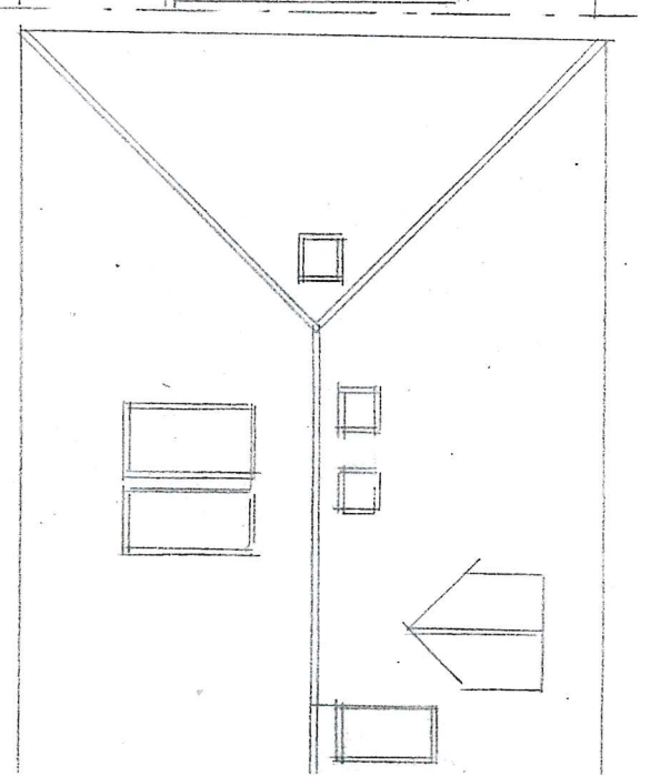
EXG ROOF PLAN
