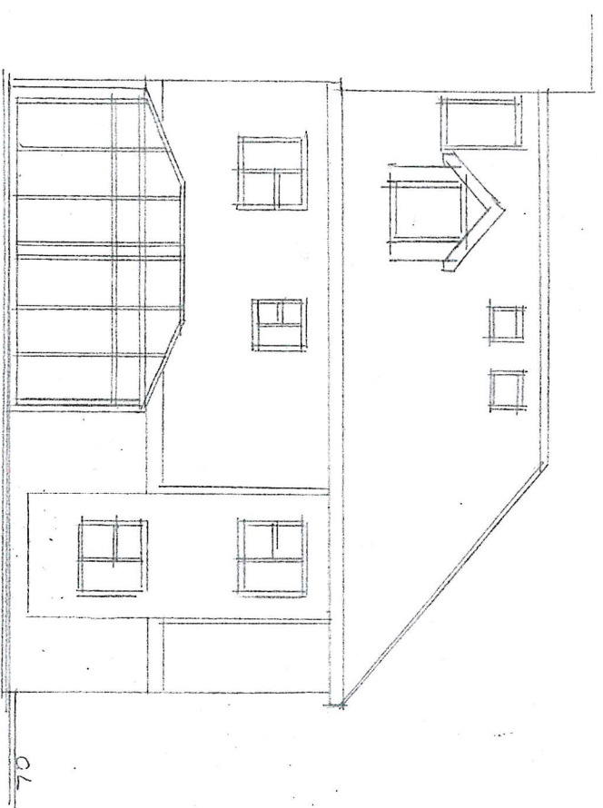
EXG WEST (REAR) ELEV
