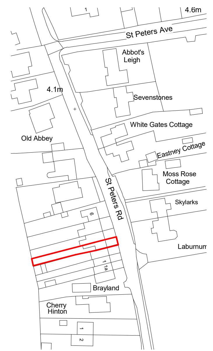
1 Location Plan 1 : 1250
