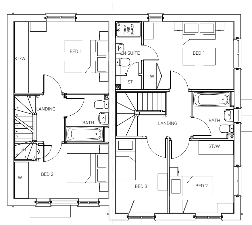
PLOT 50 FIRST FLOOR PLAN
