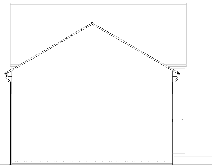
PLOT 50 SIDE ELEVATION
