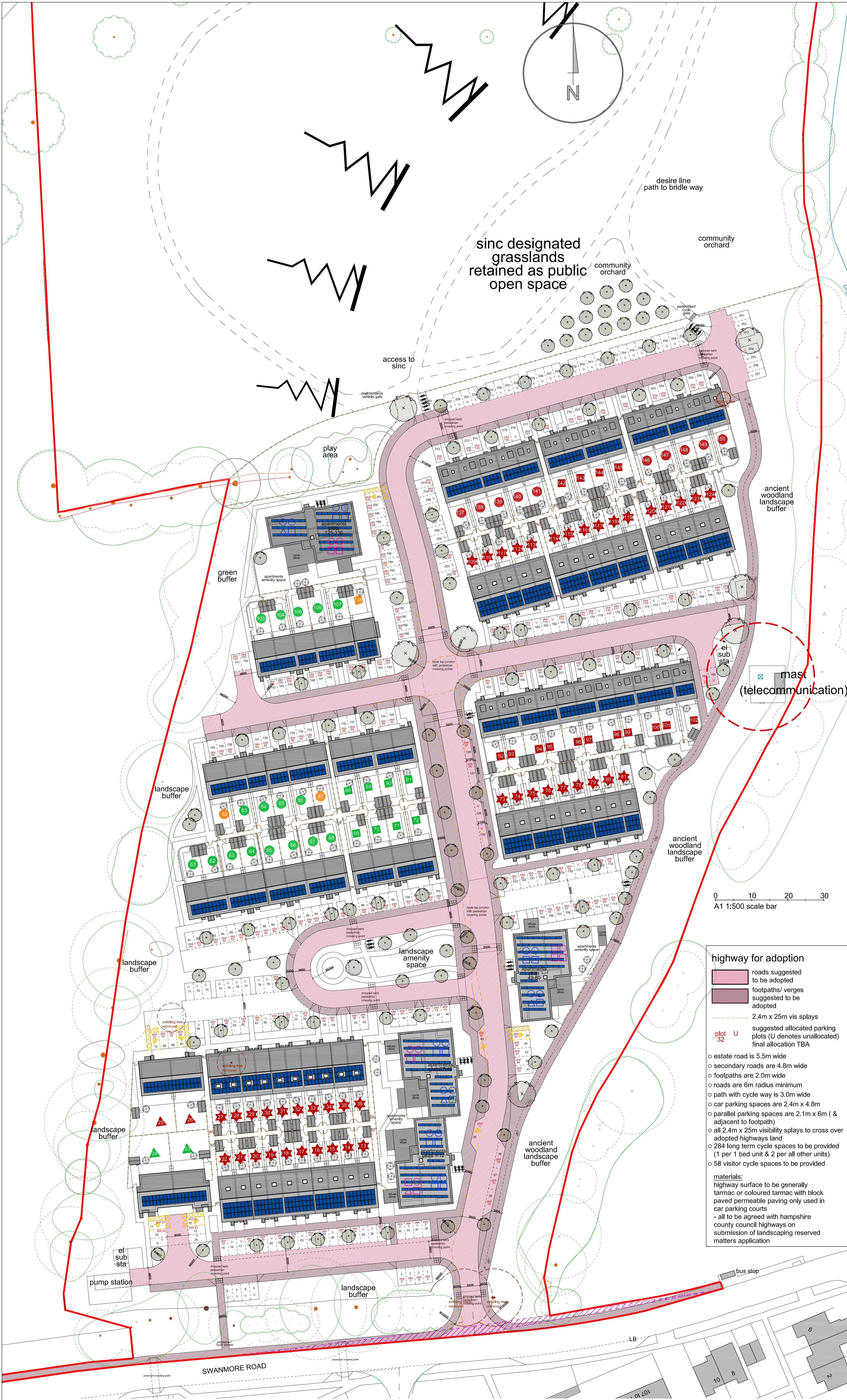
indicative adoptable highways plan (subject to agreement with hampshire county council highways)
