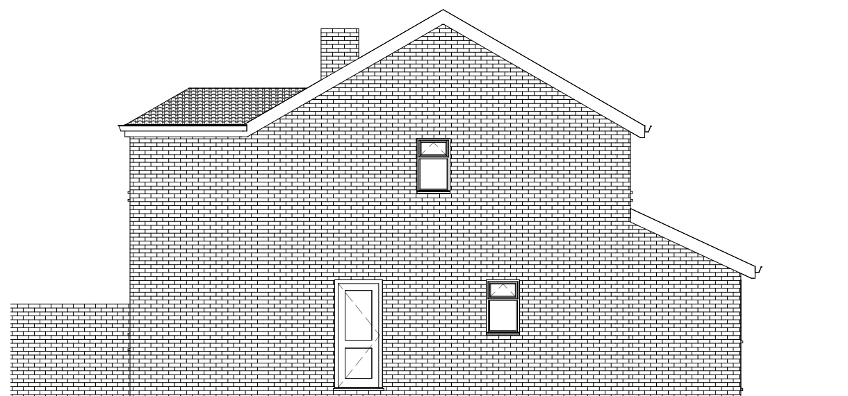
3 South Elevation 1 : 100
