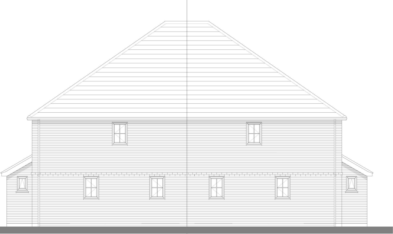
Side Elevation
