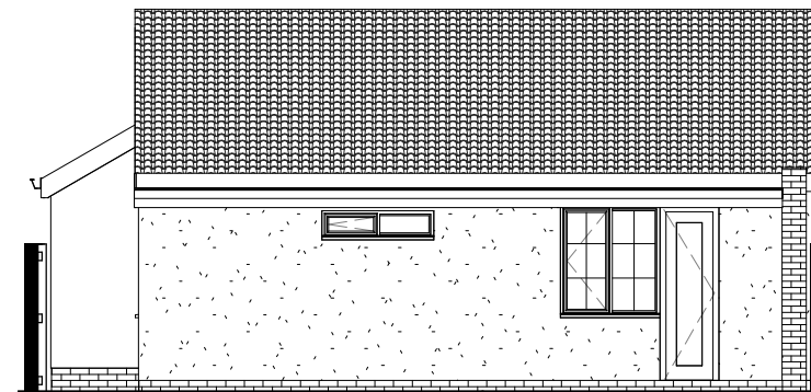
4 West Elevation 1 : 100
