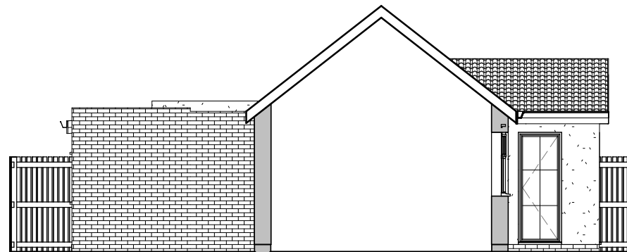
3 South Elevation 1 : 100
