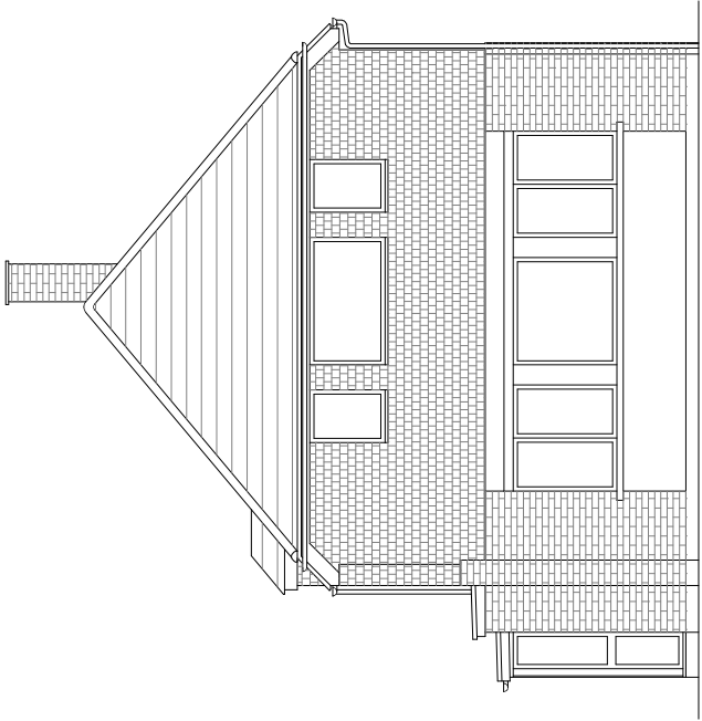
PROPOSED FRONT ELEVATION (No changes)
