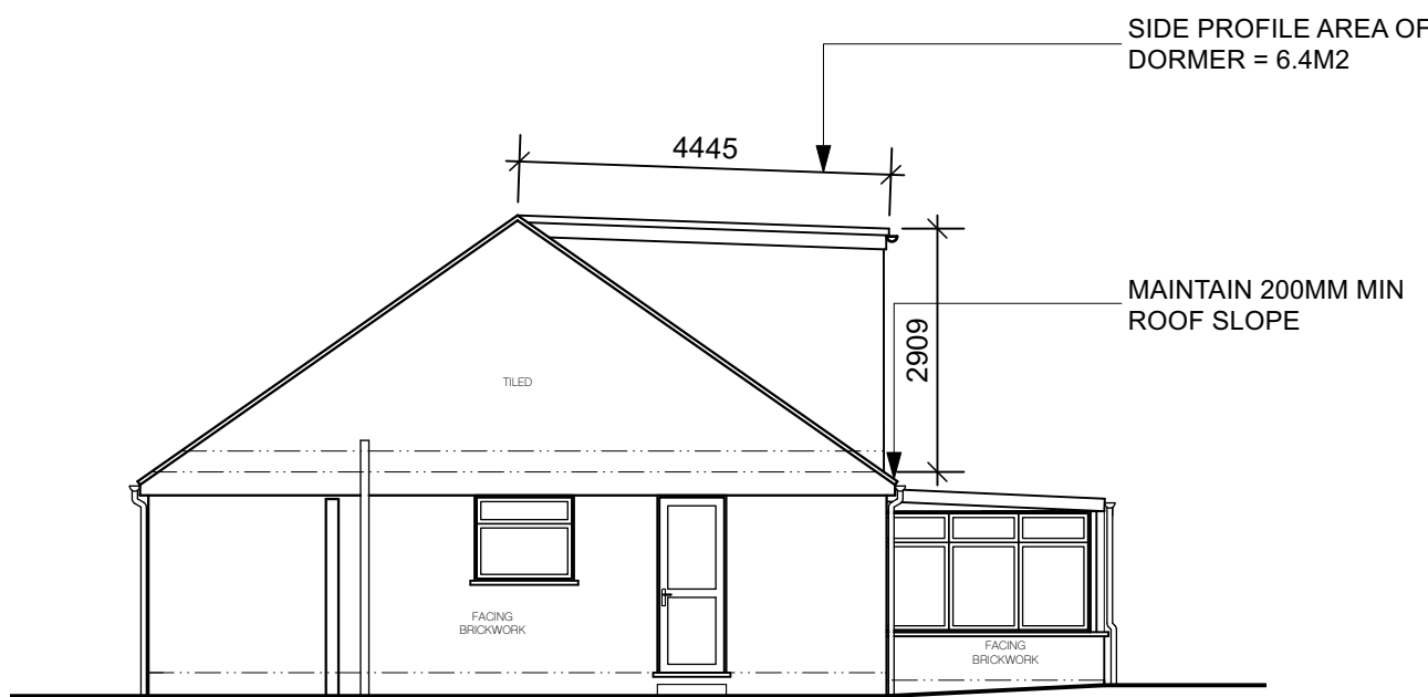
9 Proposed South Elevation Scale: 1:100
