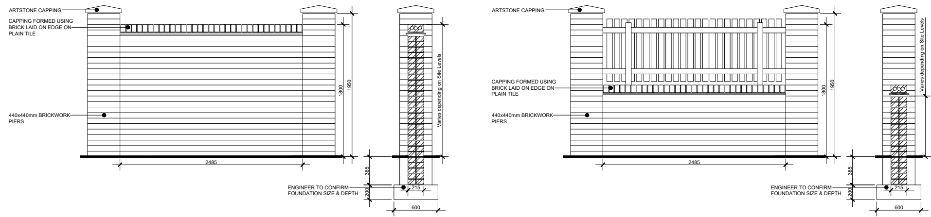
1800mm Brick Wall with Brick Piers 1800mm Dwarf Brick Wall with Brick Piers and timber panel infill
