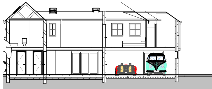
2 East West Site Section 1 : 200
