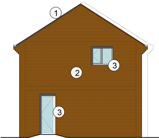
proposed north (side) elevation
