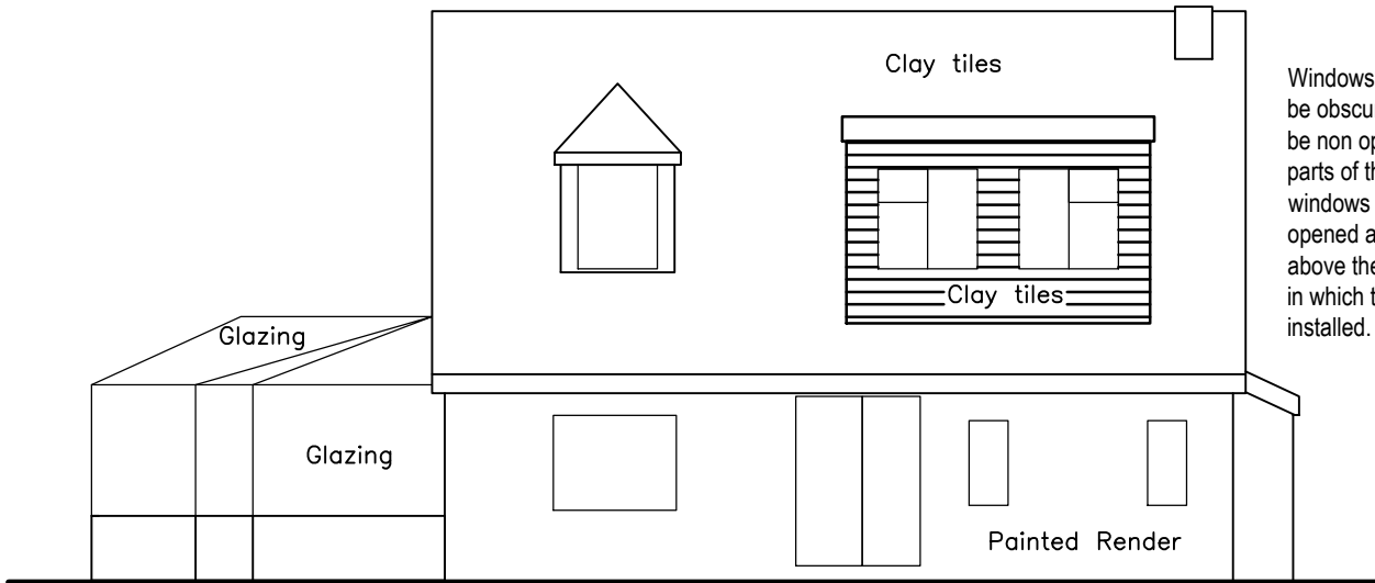
PROP SIDE ELEVATION
