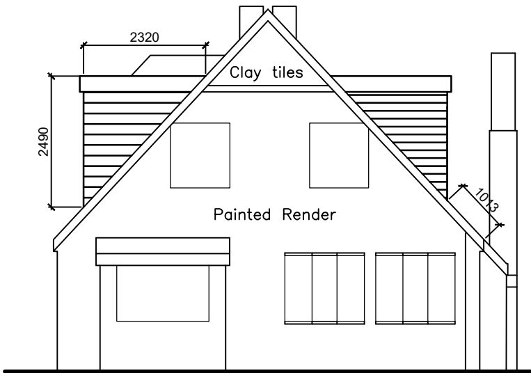
PROP FRONT ELEVATION
