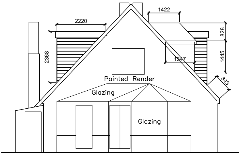
PROP REAR ELEVATION
