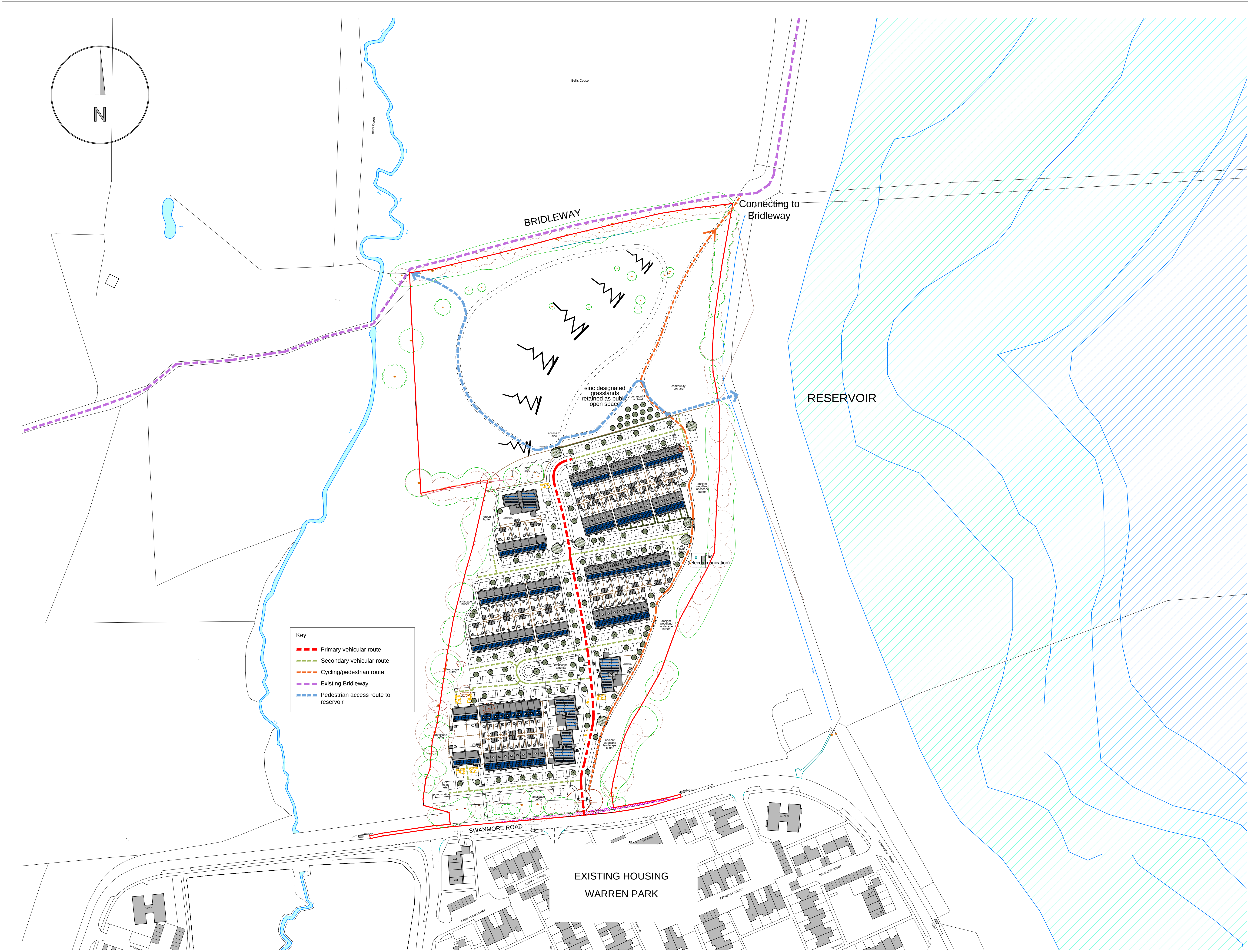
site context plan
