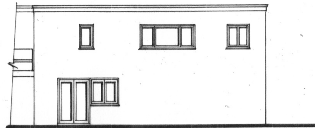
north elevation as proposed
