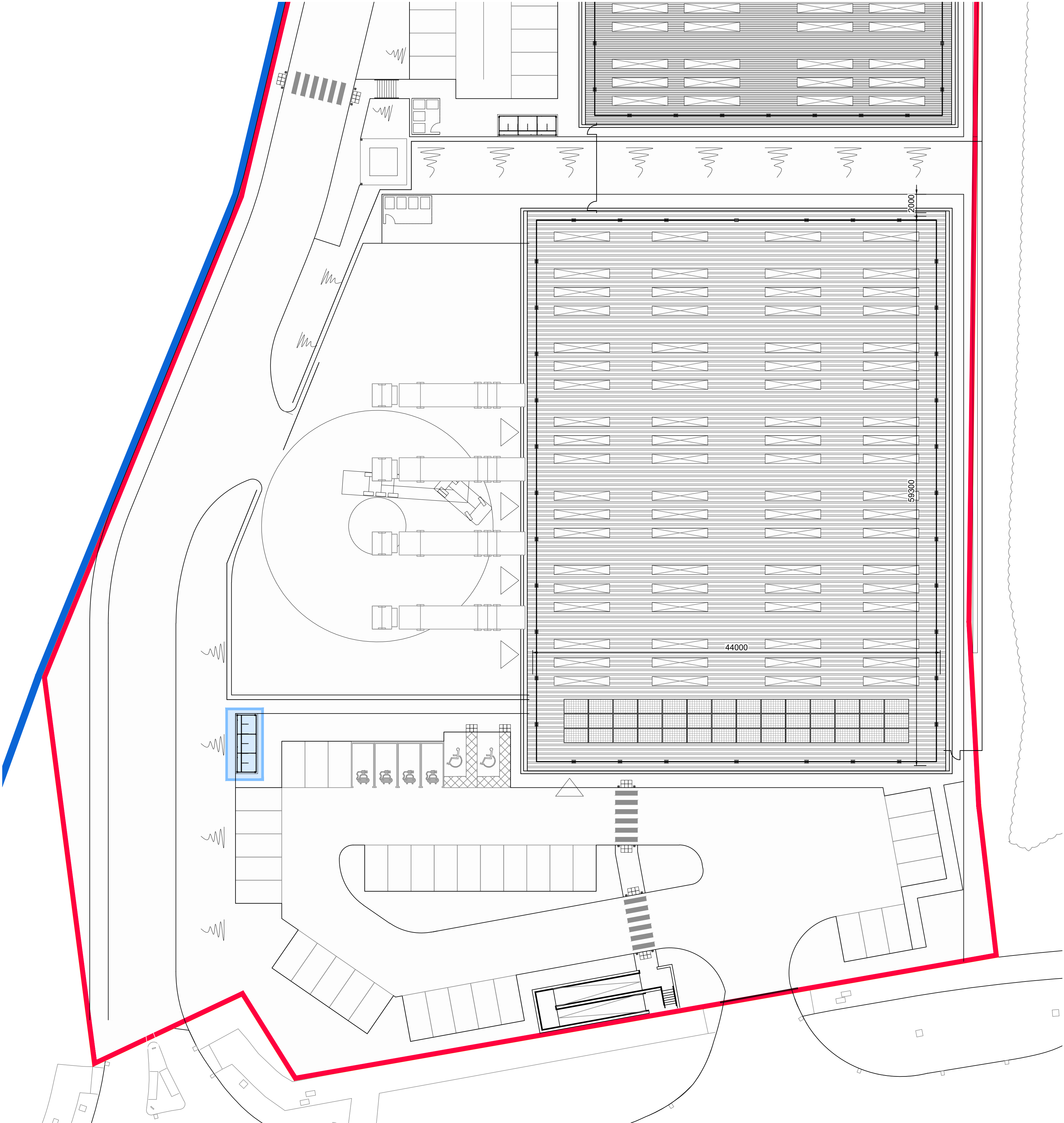
Site Layout Scale 1:250
