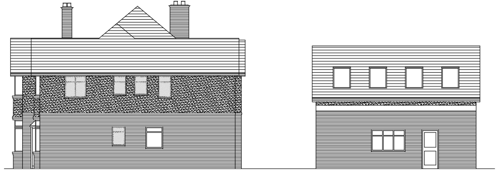
South Elevation (Side) 1:100 @A1
