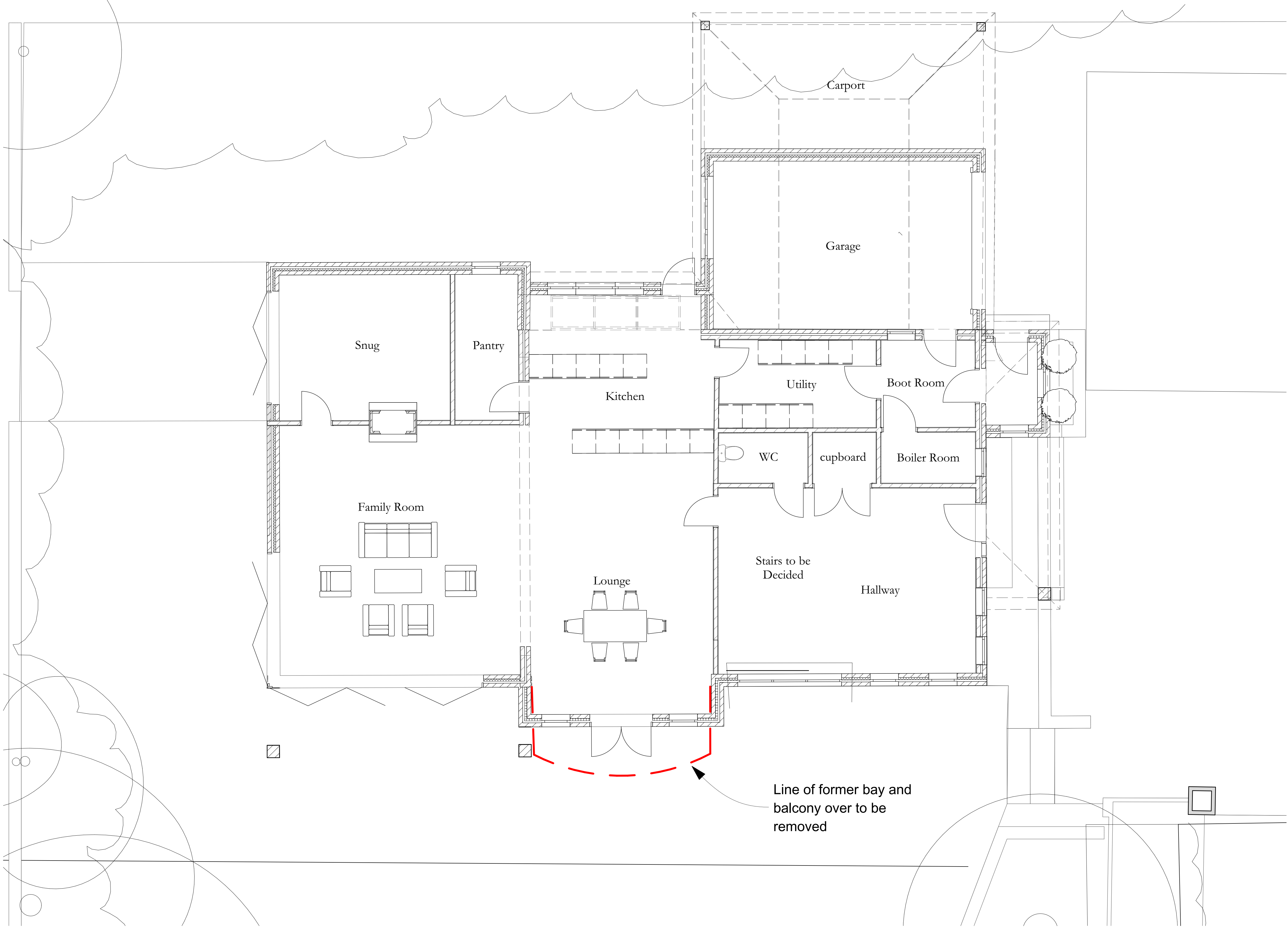
Ground Floor 1:50
