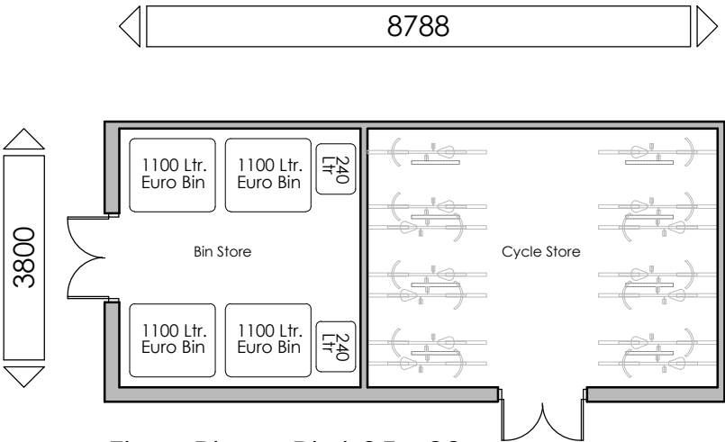
Floor Plan - Plot 85 - 93 Plot 94 - 102
