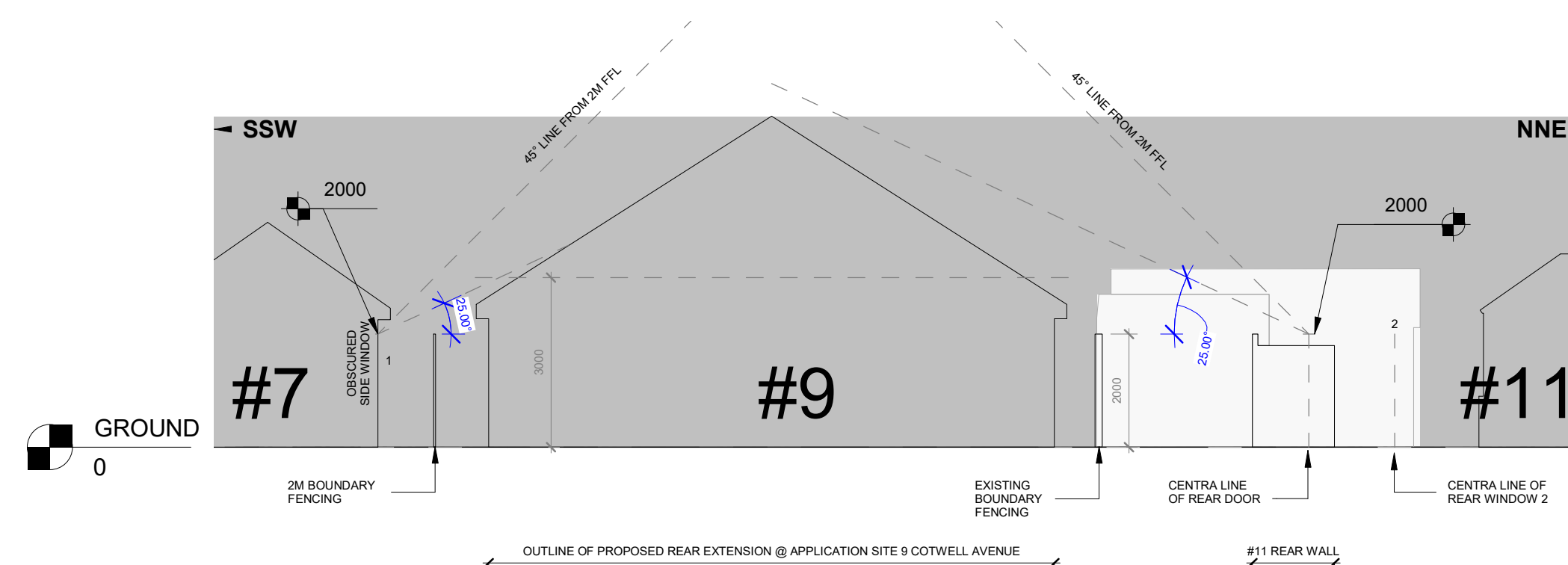
HORIZONTAL TESTING LOOKING WEST (REAR) 1 : 100
