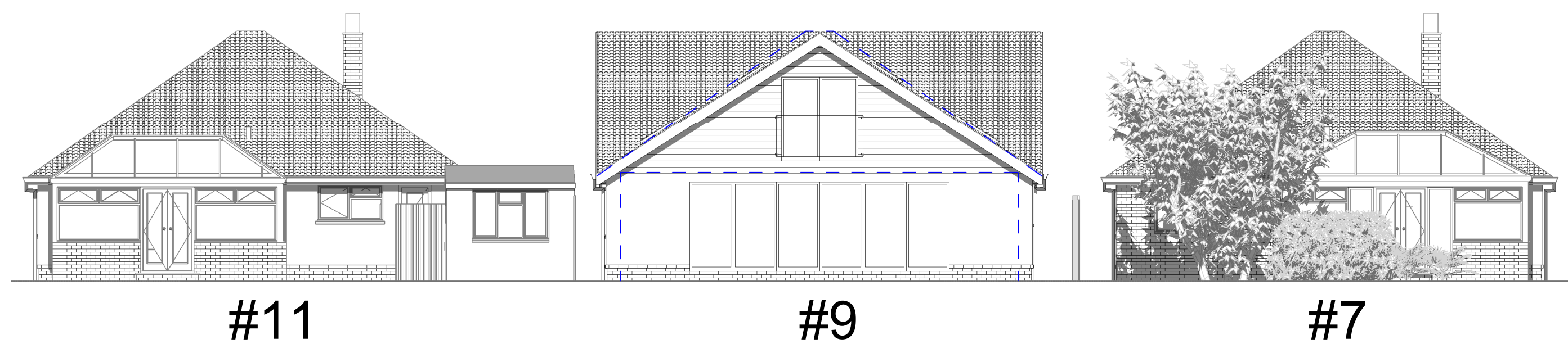
REAR SCENE 1 : 100
