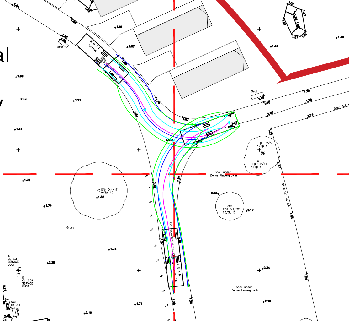
Turning Head Vehicle Path (NTS)
