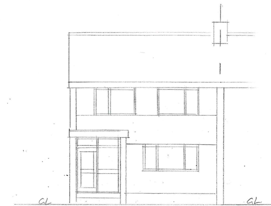
EXG FRONT ELEVATION
