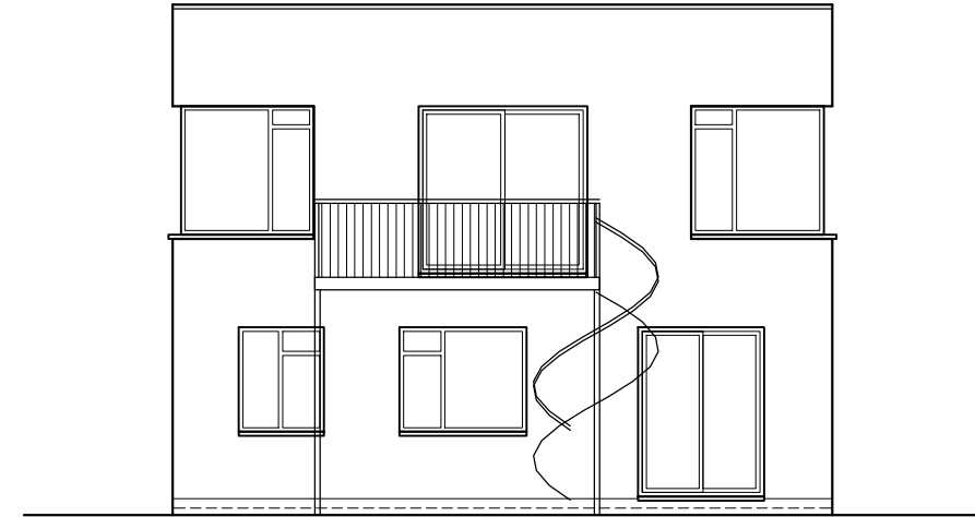
REAR (SE)
