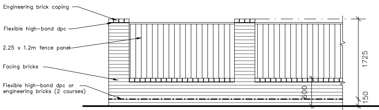
BRICK & PANEL WALL DETAIL 1:50 (External face shown towards public areas)
