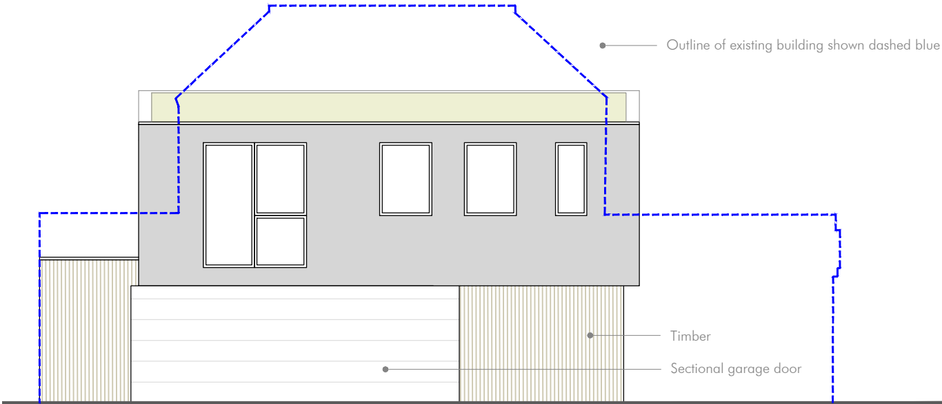
South Elevation
