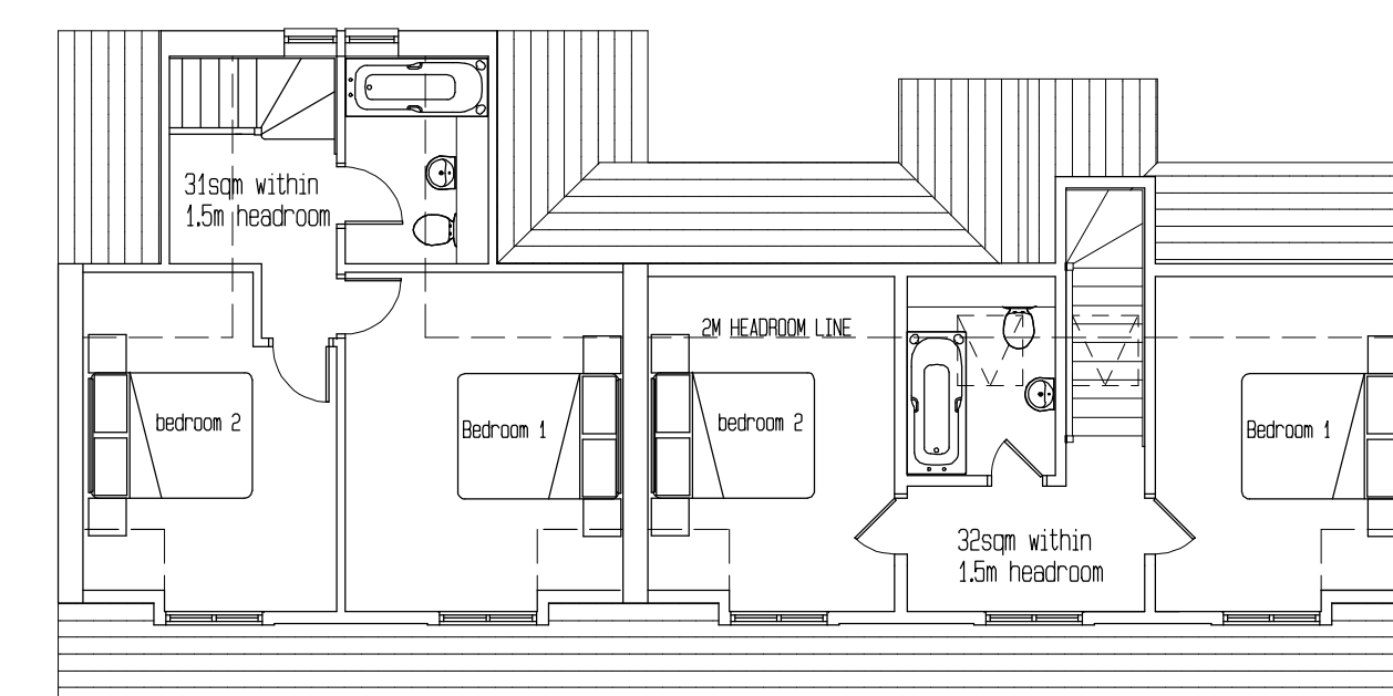
First Floor Plan Plots 3 & 4
