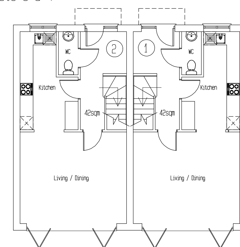
Ground Floor Plan Plots 1 & 2
