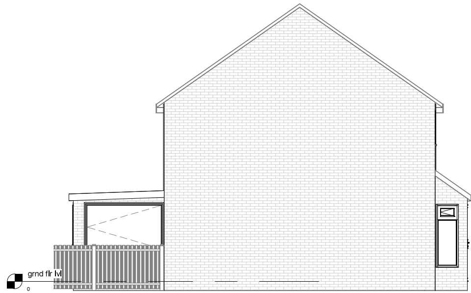
Existing Elevation-Left side
