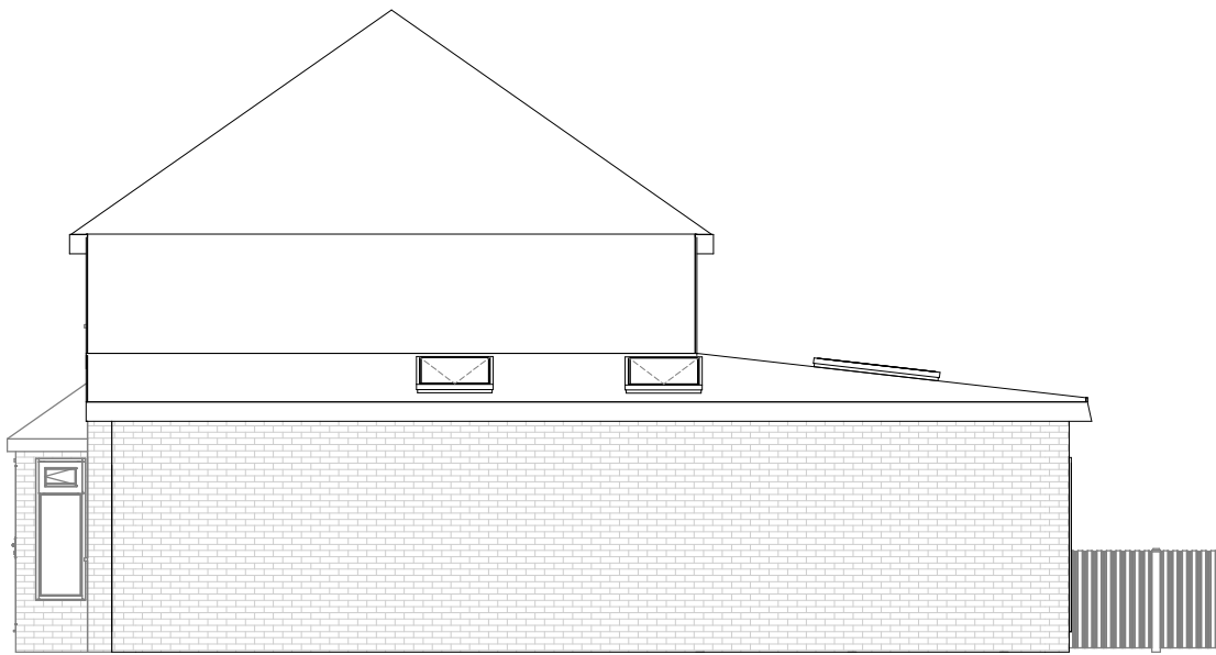
Proposed Elevation-Right side
