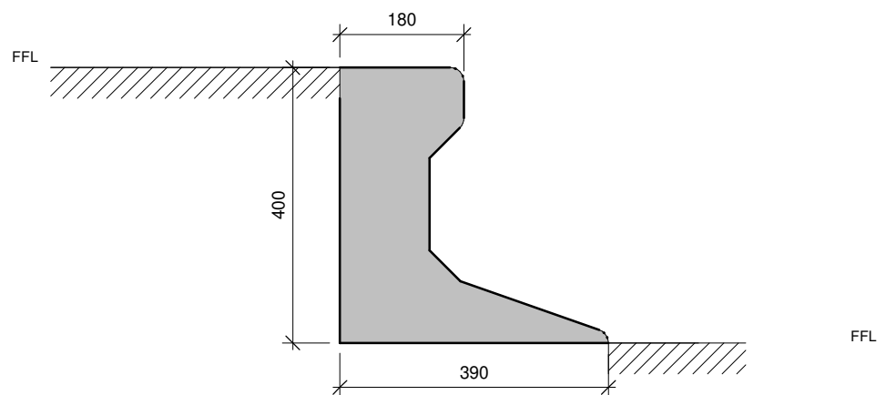
KT02 400 x 390mm PRECAST CONCRETE TRIEF KERB
