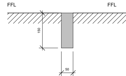
KT03 150 x 80mm PRECAST CONCRETE FIN KERB
