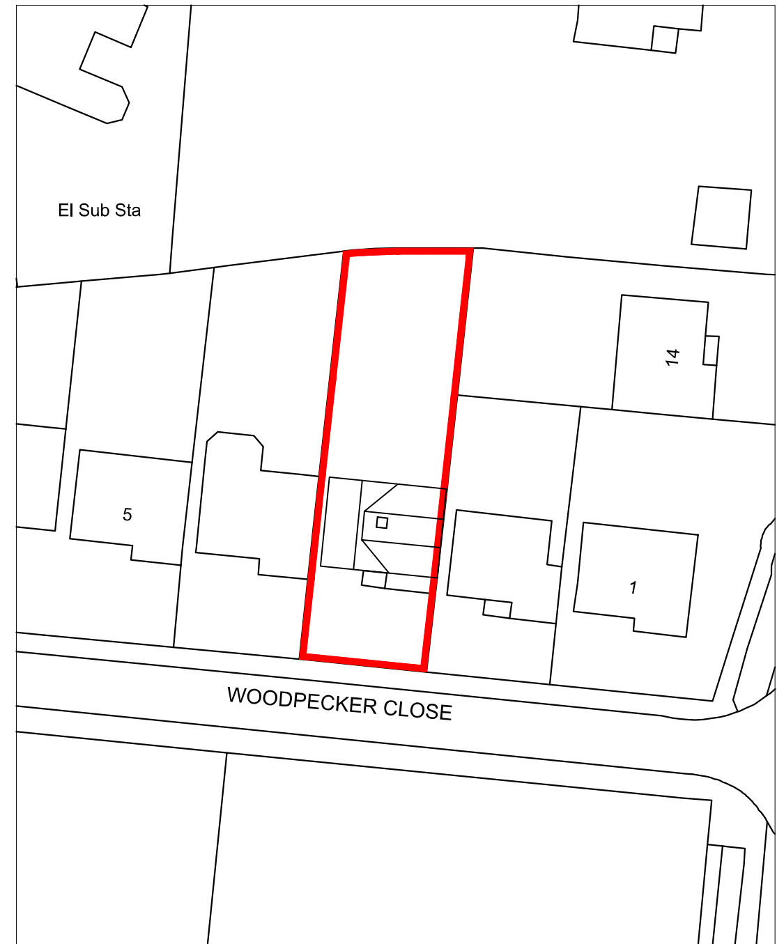
Block Plan: 1:500
