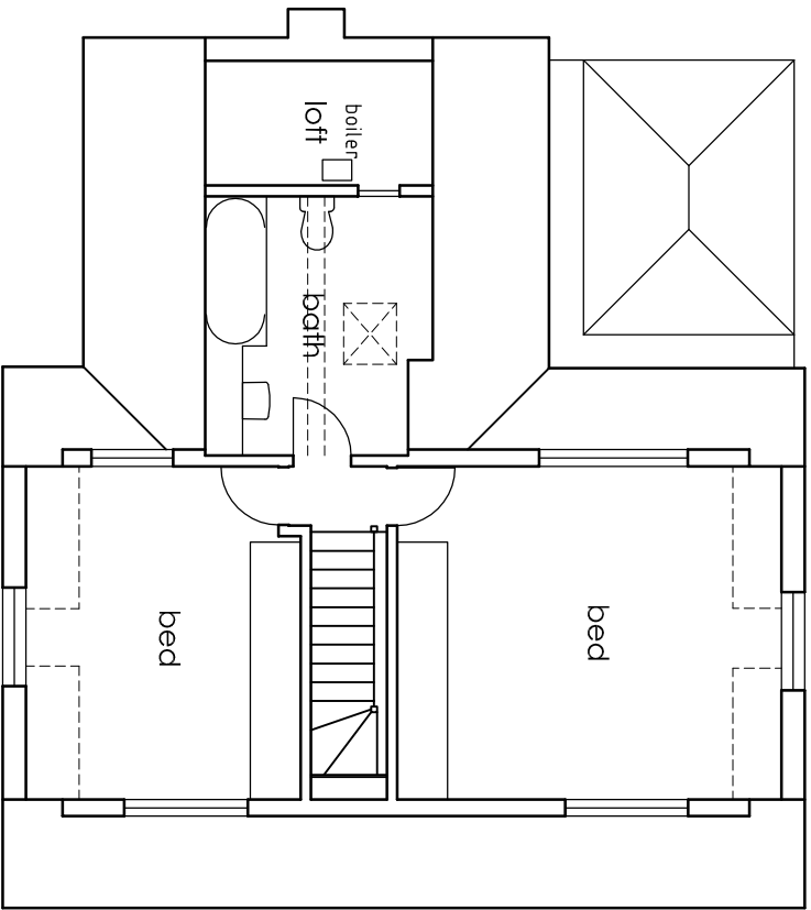
First 1:100
