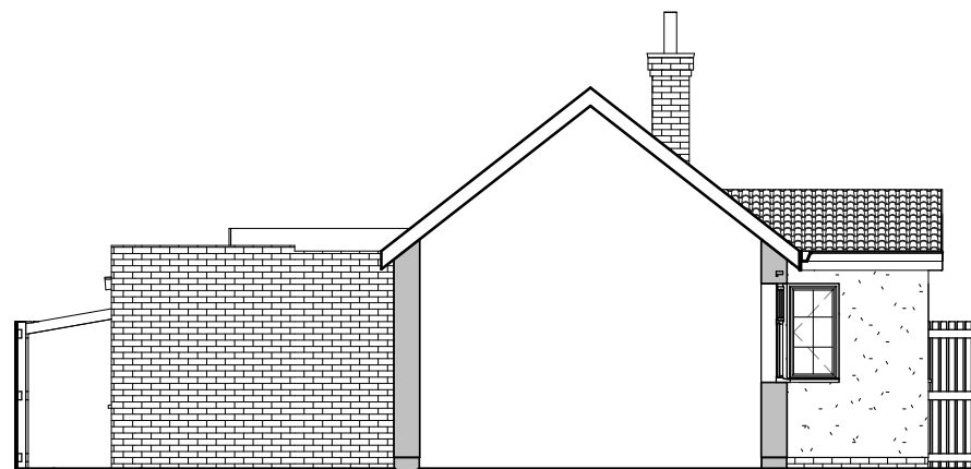
3 South Elevation 1 : 100
