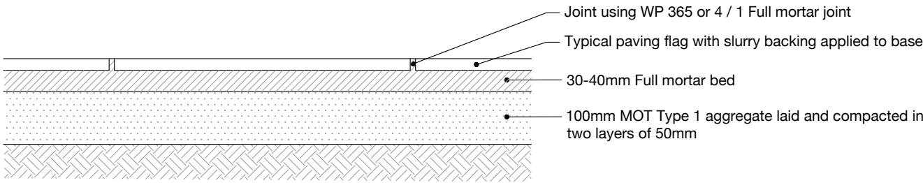
Indian Standstone Paving Installation Detail
