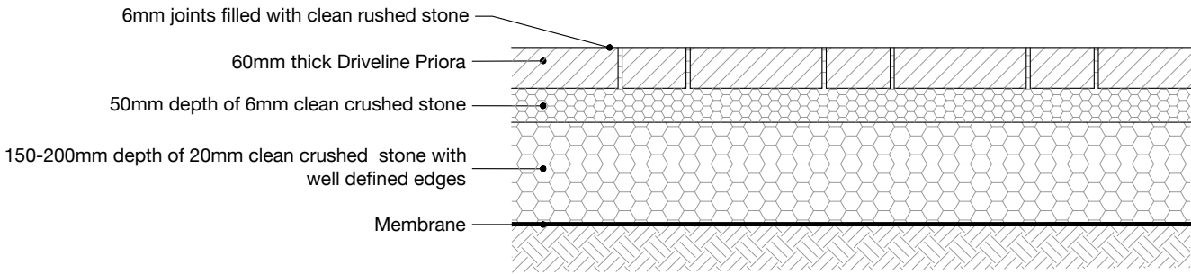
Driveline Piora Paving Installation Detail
