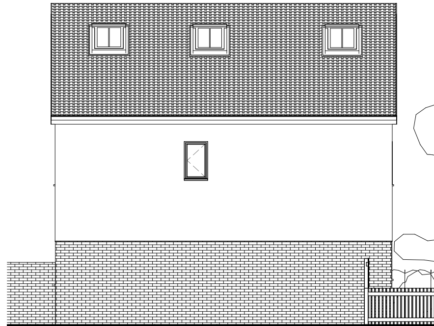
1 East Elevation 1 : 100
