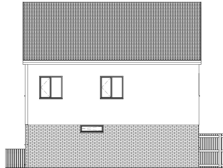
4 West Elevation 1 : 100
