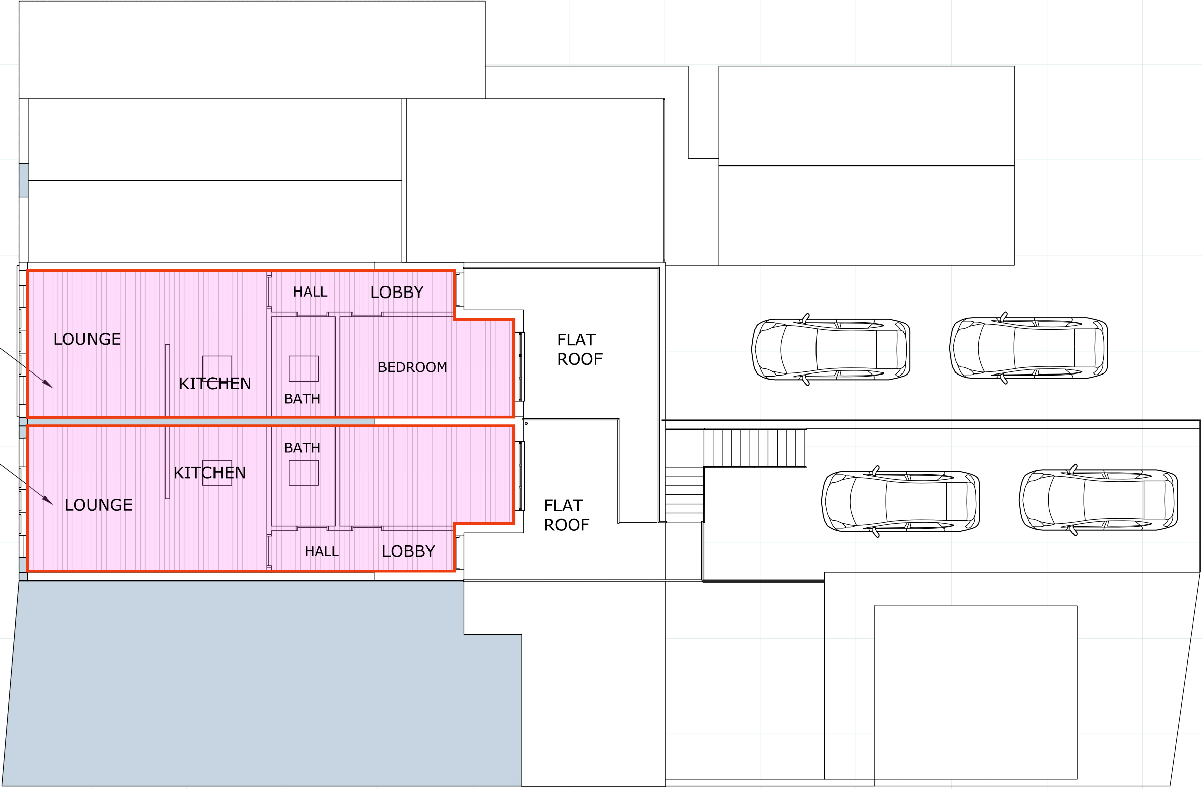
PROPOSED FIRST FLOOR PLAN (NEW FLATS)
