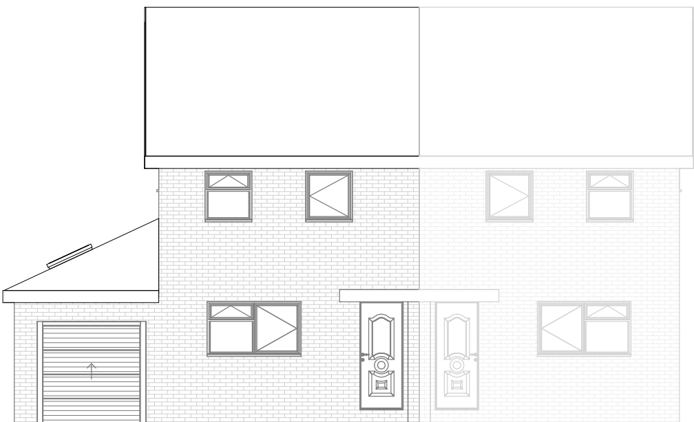
Proposed Elevation-Front
