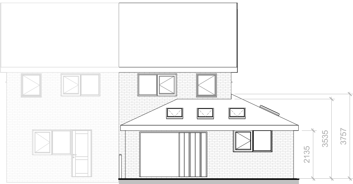
Proposed Elevation-Rear
