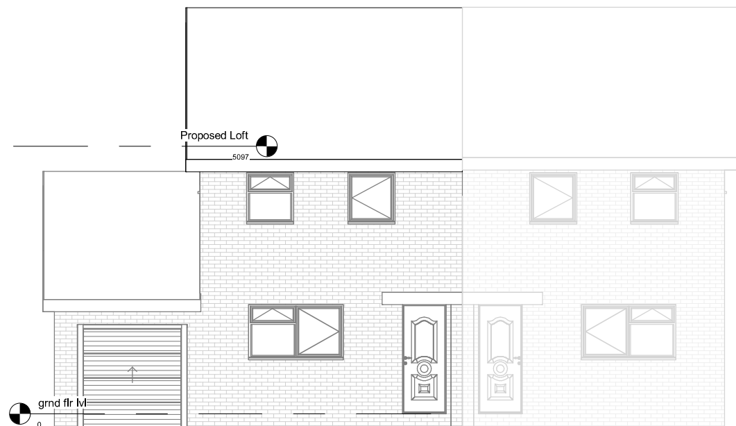
Existing Elevation-Front
