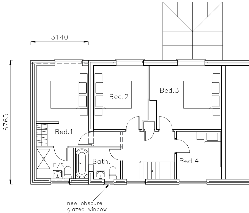
FIRST FLOOR
