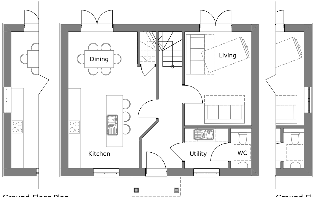
Ground Floor Plan to Plot 59 Ground Floor Plan to Plots 59&63
