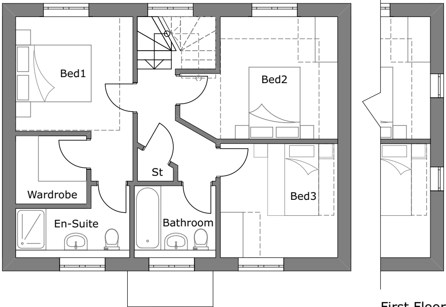
First Floor Plan First Floor Plan to Plots 59&63
