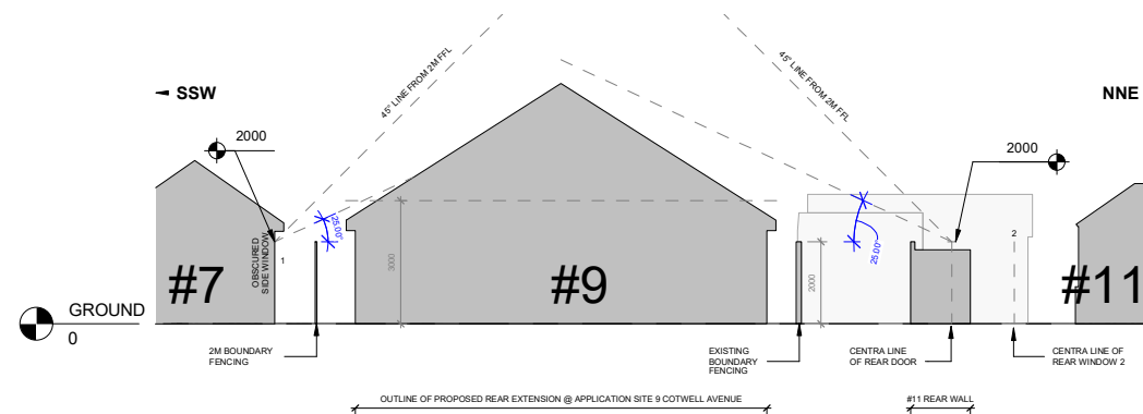
HORIZONTAL TESTING LOOKING WEST (REAR) 1 : 100
