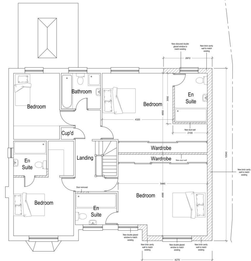
Proposed First Floor Plan Scale 1:50
