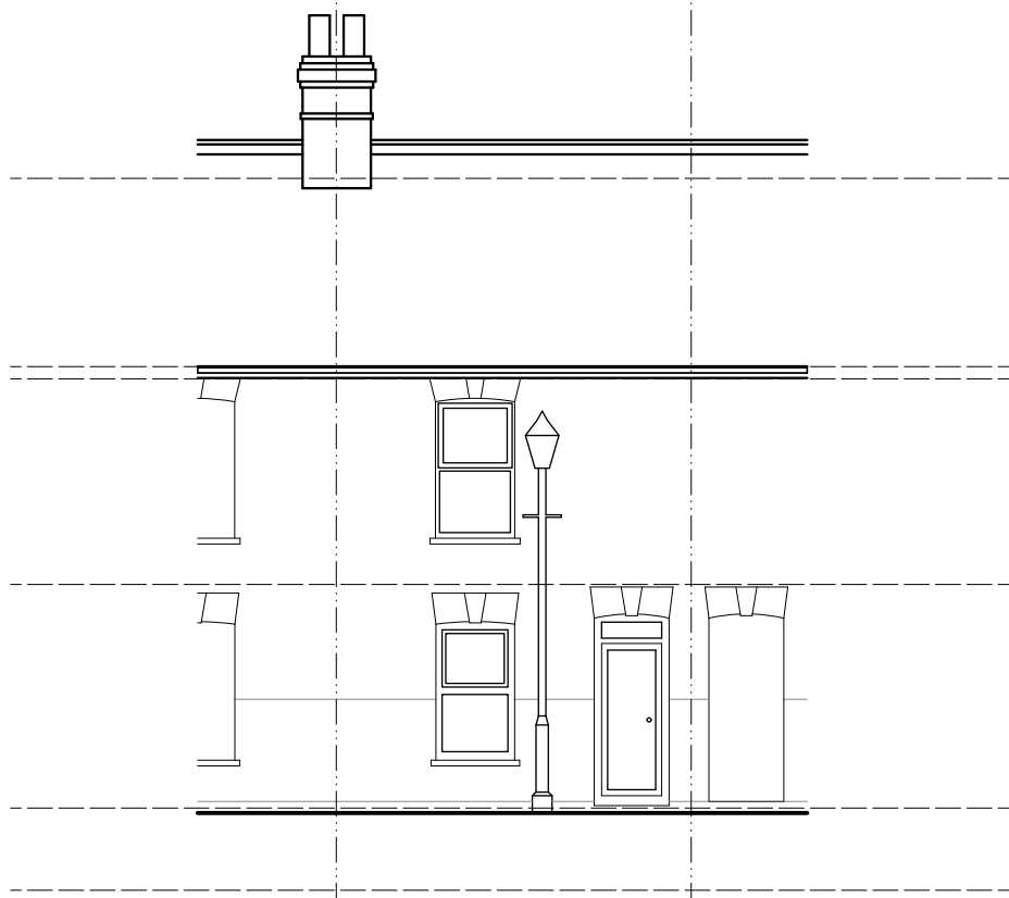
2 Existing Front Elevation Scale: 1:100
