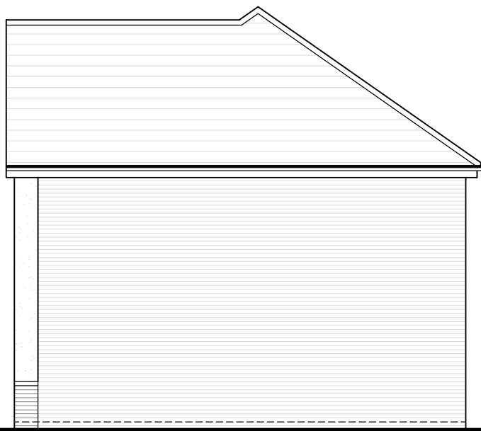
Side Elevation
