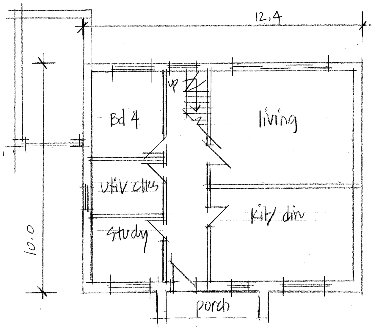
GROUND FLR
