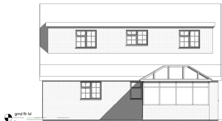
Existing Elevation-Rear
