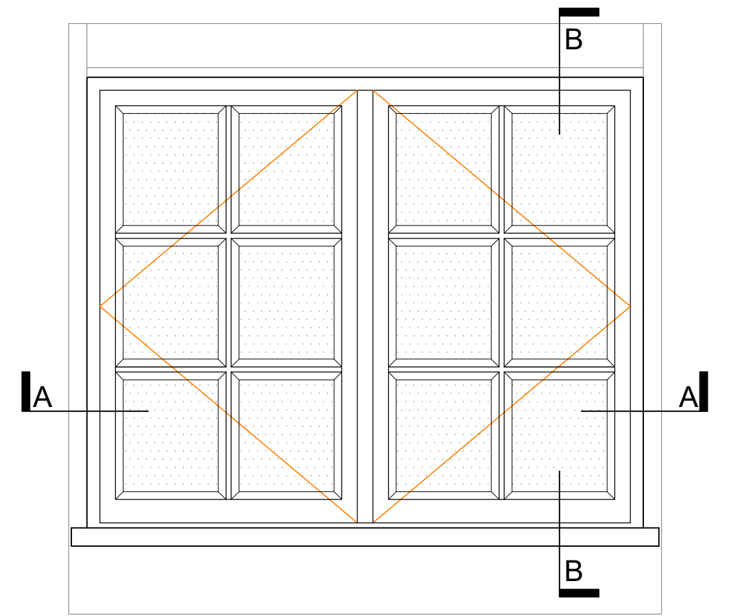
WINDOW DETAILS W1.08 @1:10
