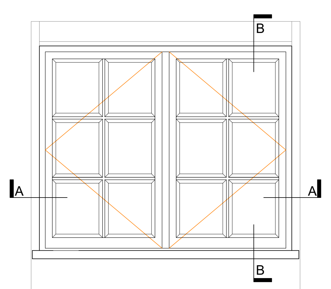
WINDOW DETAILS W1.09 @1:10
