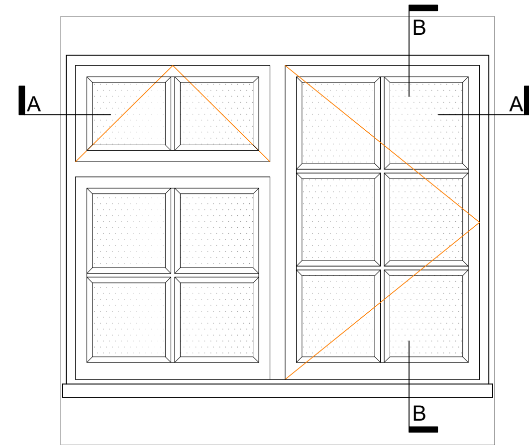
WINDOW DETAILS W1.10 @1:10
