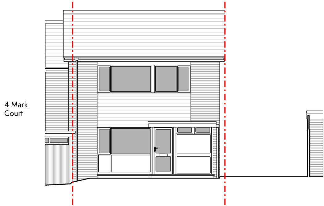
Front (South) Elevation
