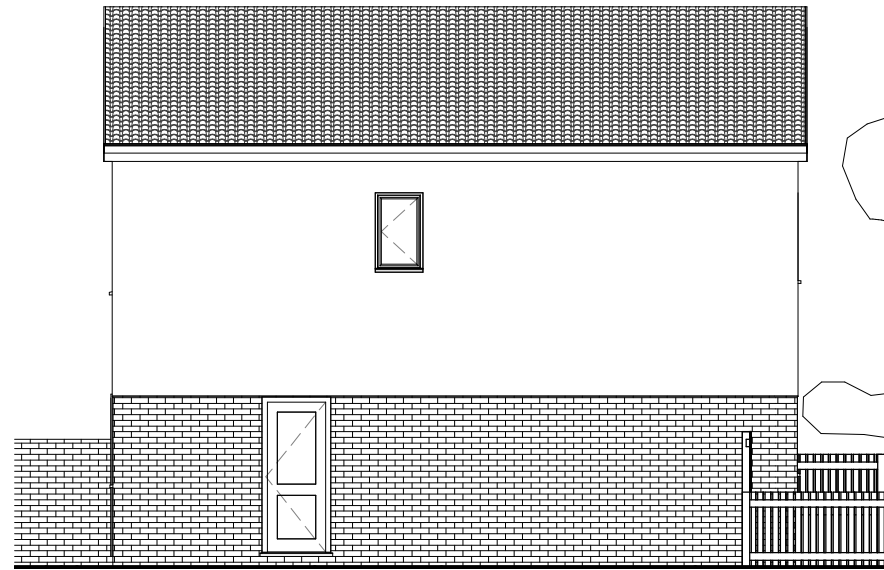
1 East Elevation 1 : 100
