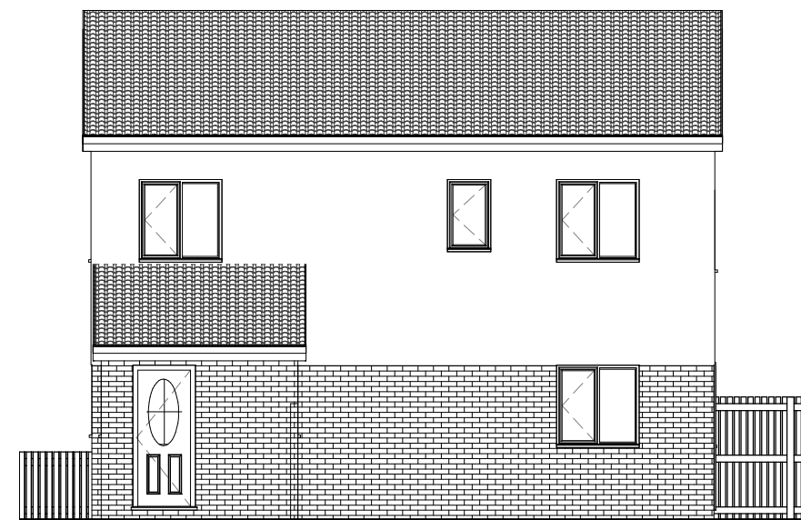
4 West Elevation 1 : 100
