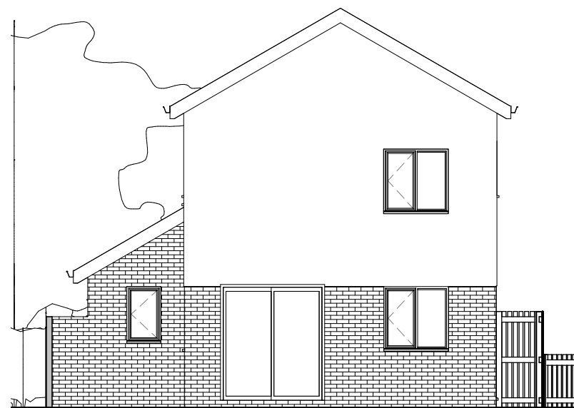
3 South Elevation 1 : 100
